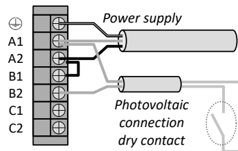
Dry contact inlet diagram
